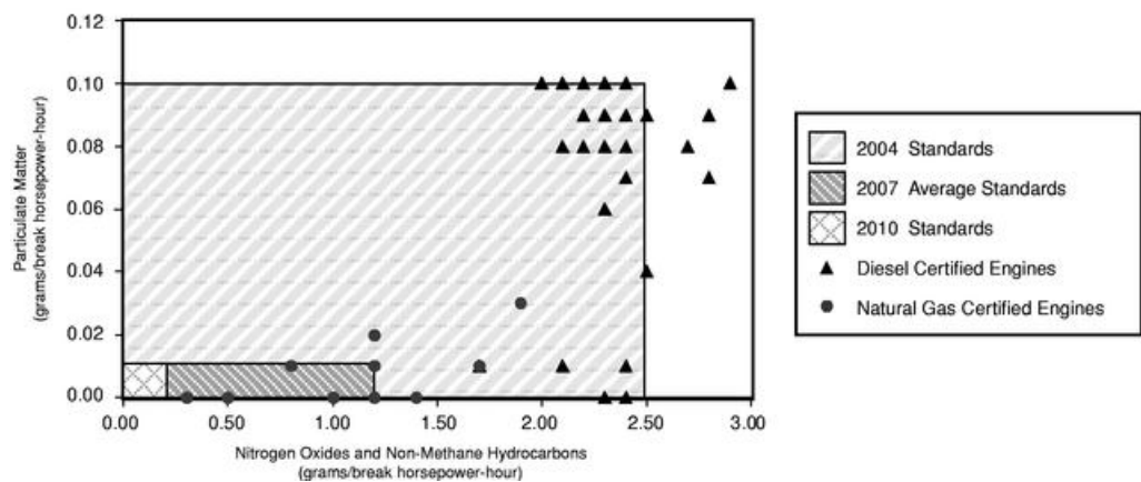
South Coast Air Quality Management District Study: 2006 On-Road Heavy-Duty Engine Certifications Based on Federal Emissions Standards (as of May 19, 2006)
